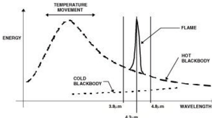
Fig. 3. Blackbody Rejection
